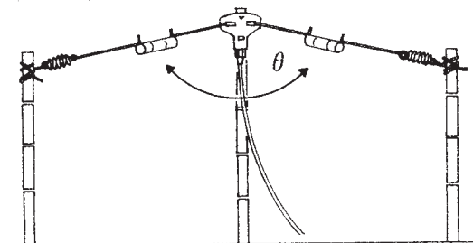
Inverted V ( \theta = 120^\circ )
